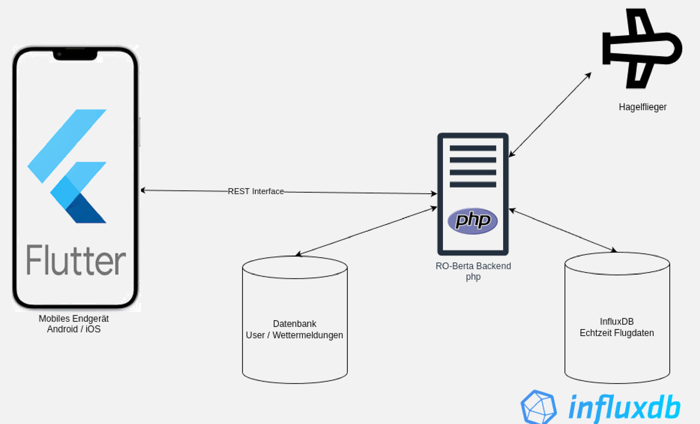
Fig. 6: Architecture diagram
